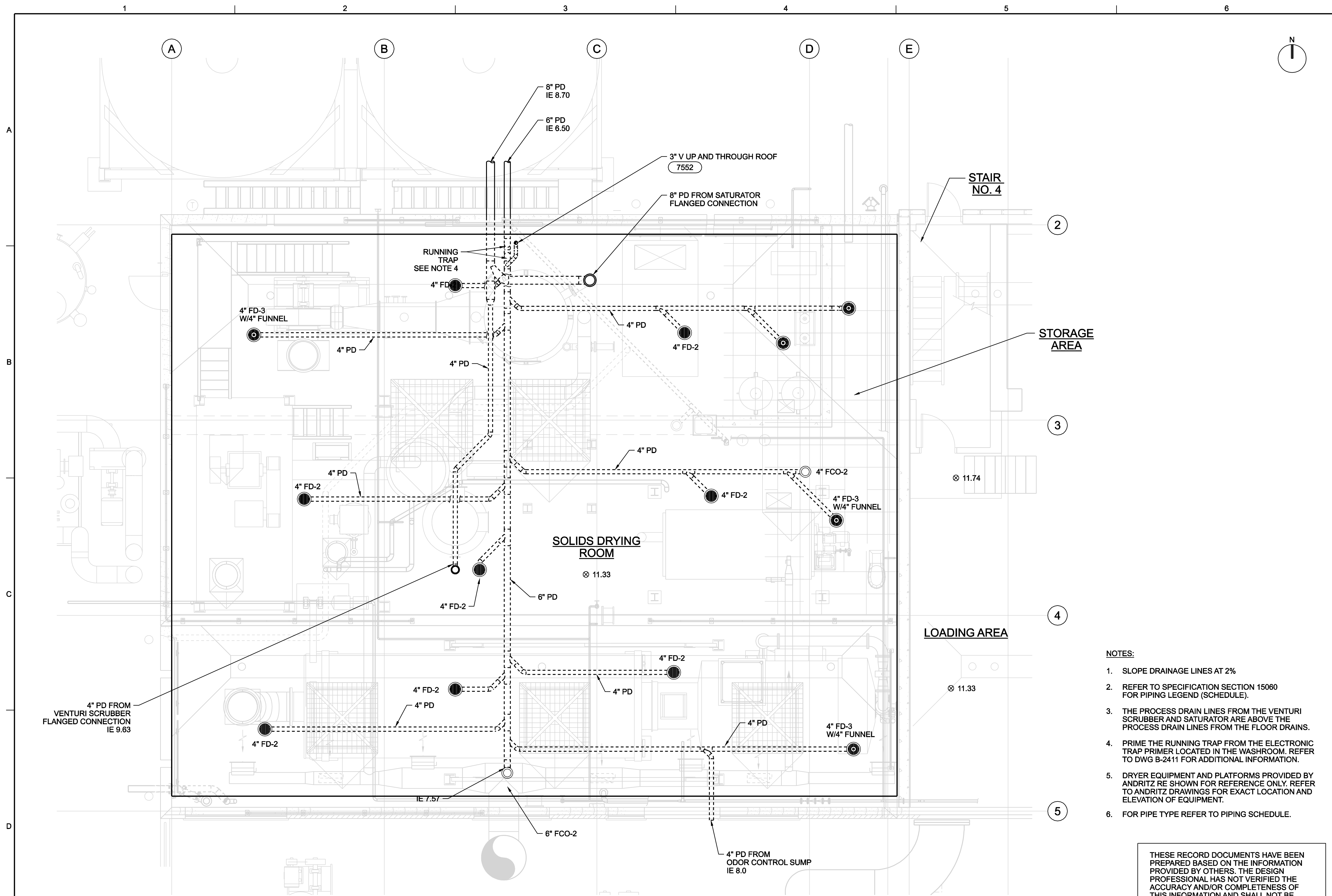
MAIN FLOOR PLAN 1/4"=1'-0"
