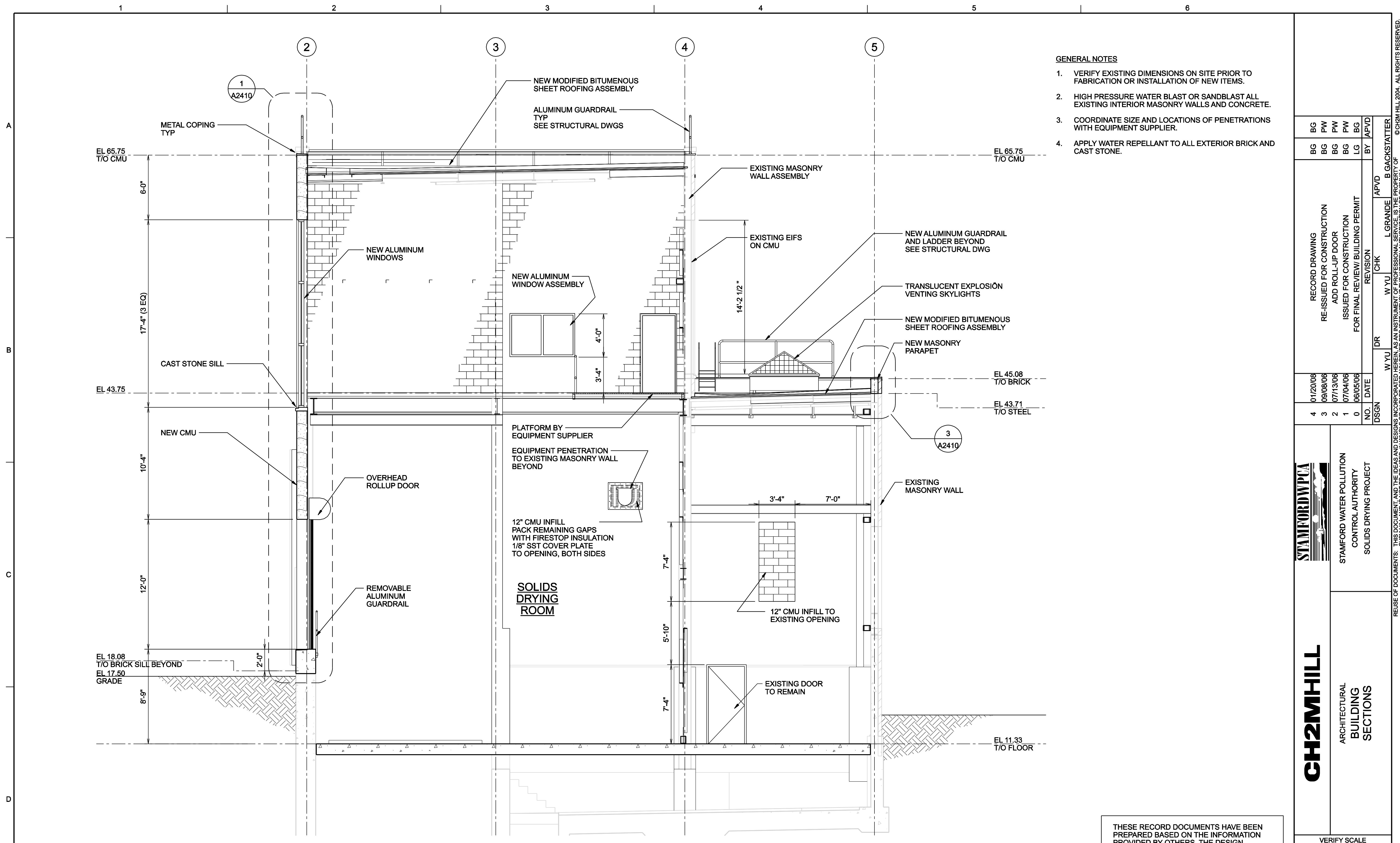
A BUILDING SECTION A 1/4"=1'-0" A2400
