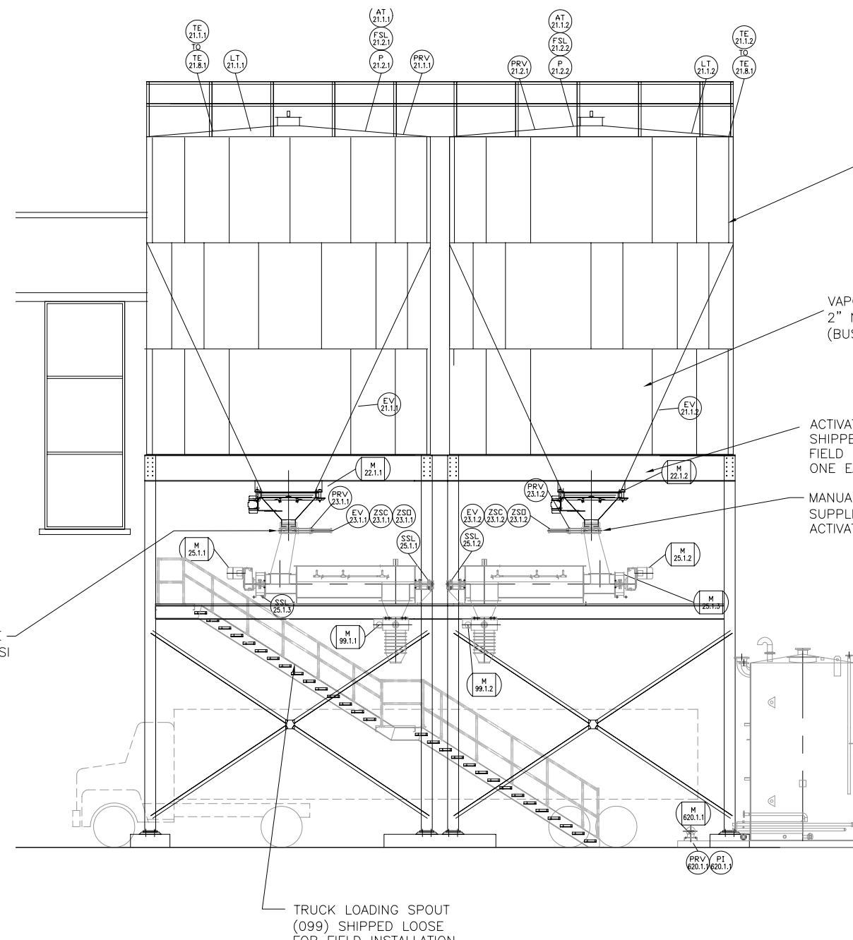
ELEVATION VIEW
