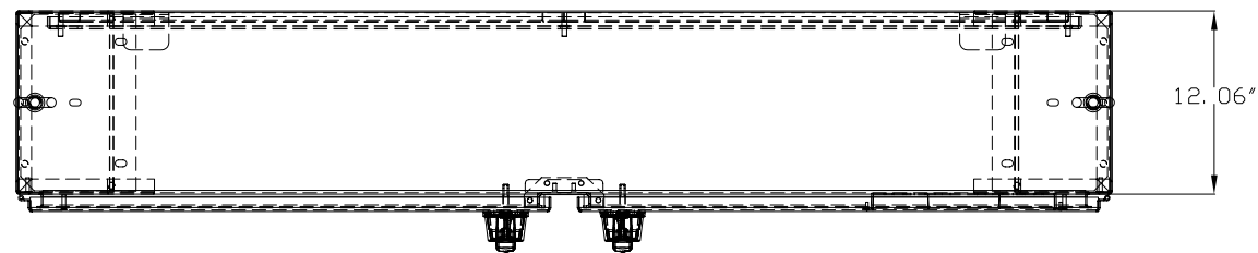
BOTTOM VIEW
